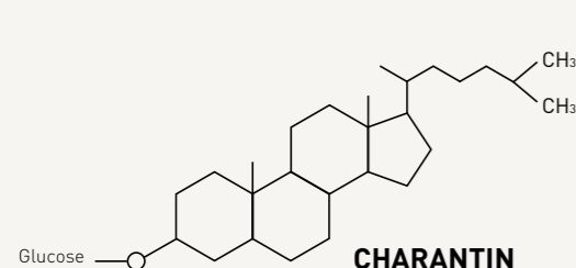
Structural formula of some active principles of the Bitter melon phyto-complex.
